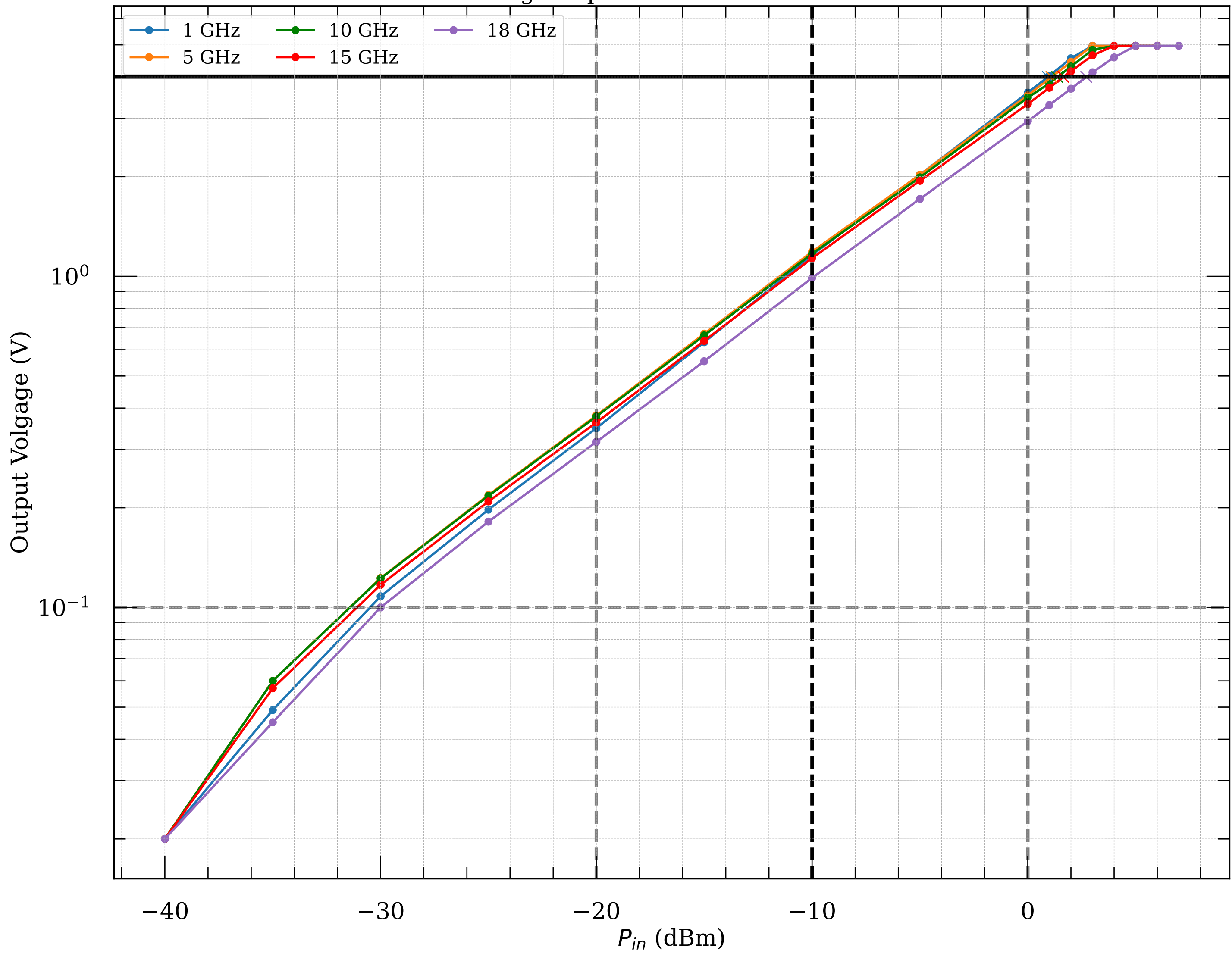
Measured voltage-to-power curve of detector module062
